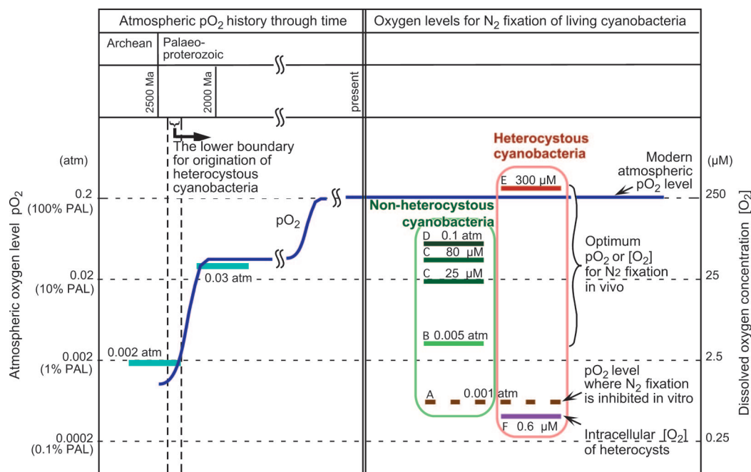
Fig. 3. The geochemical record of atmospheric oxygen as it relates to nitrogen fixation and the evolution of heterocystous cyanobacteria. The curve presents an estimate of atmospheric P_{O_2} through time, as constrained by paleosol (42) and \delta^{15}N isotopic (43, 44, 46) data. Numbers in Right indicate the P_{O_2} level at which in vitro nitrogenase activity is inhibited in nonheterocystous Plectonema and heterocystous Anabaena (34) (A), and P_{O_2} or [O_2] optima for in vivo nitrogenase activity of Plectonema (36) (B), nonheterocystous Gloeotheca (37) (C), Trichodesmium (38) (D), and Anabaena (39) (E). F indicates the intracellular [O_2] of Anabaena heterocysts. The [O_2] (the left vertical axis) corresponds to P_{O_2} (right axis) when [O_2] is 250 \mu M in air-saturated water. PAL, present atmospheric level.
